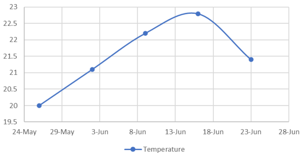
Temperature
