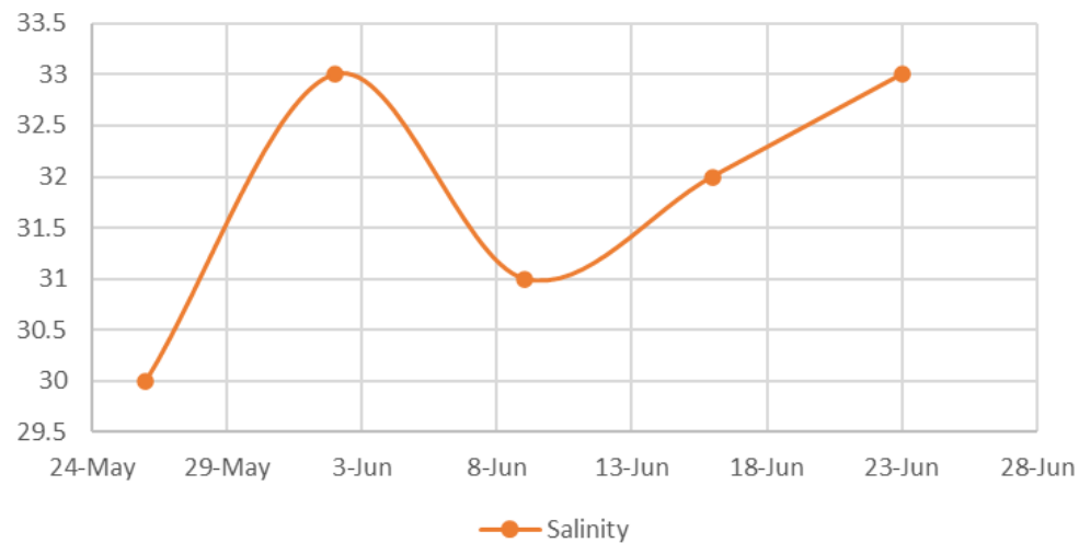
Salinity
