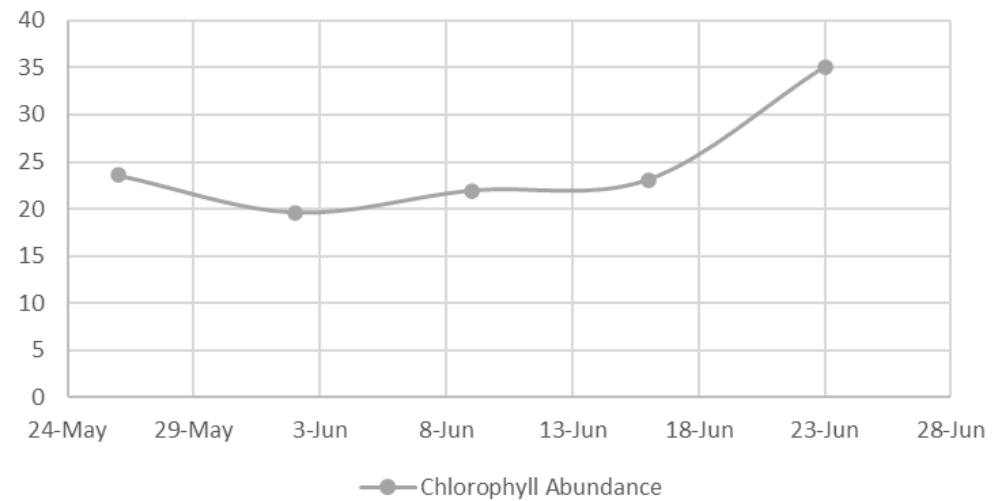
Chlorophyll Abundance
