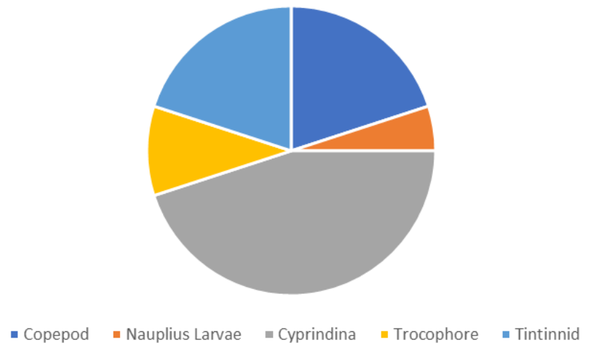
Plankton Speciation
