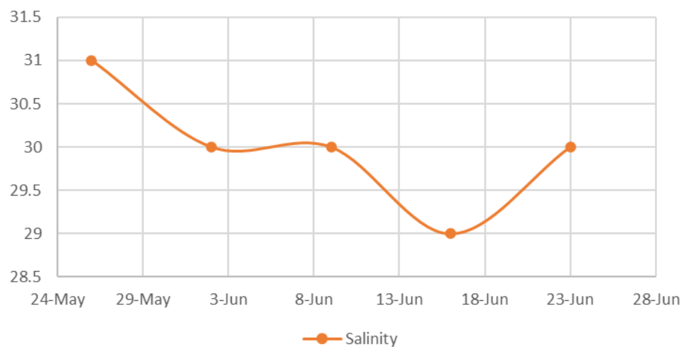
Salinity
