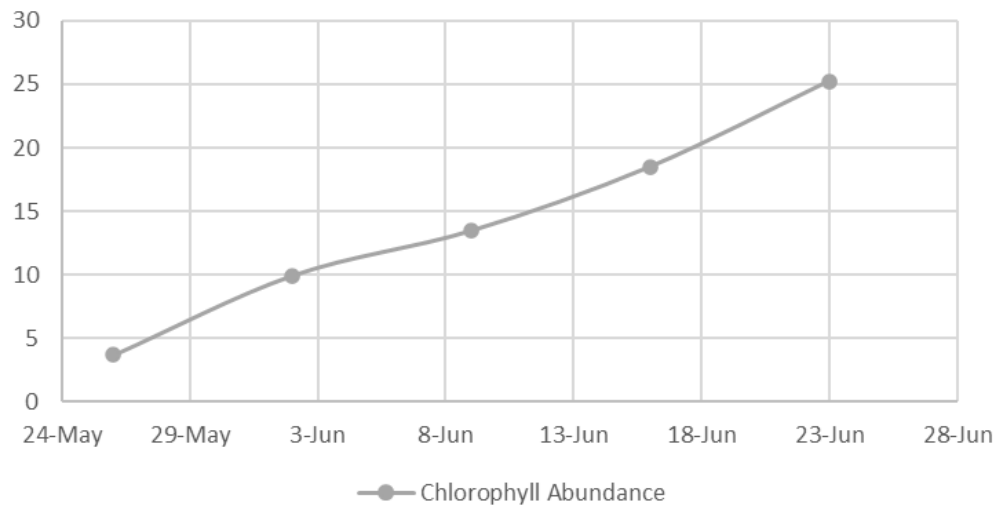
Chlorophyll Abundance
