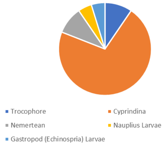
Plankton Speciation
