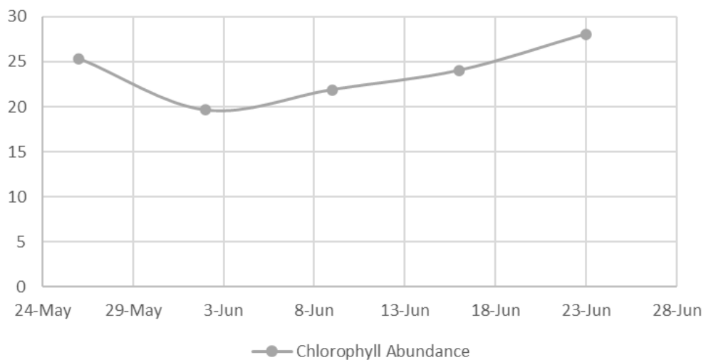
Chlorophyll Abundance
