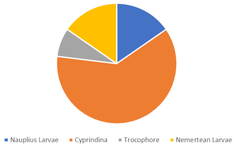
Plankton Speciation
