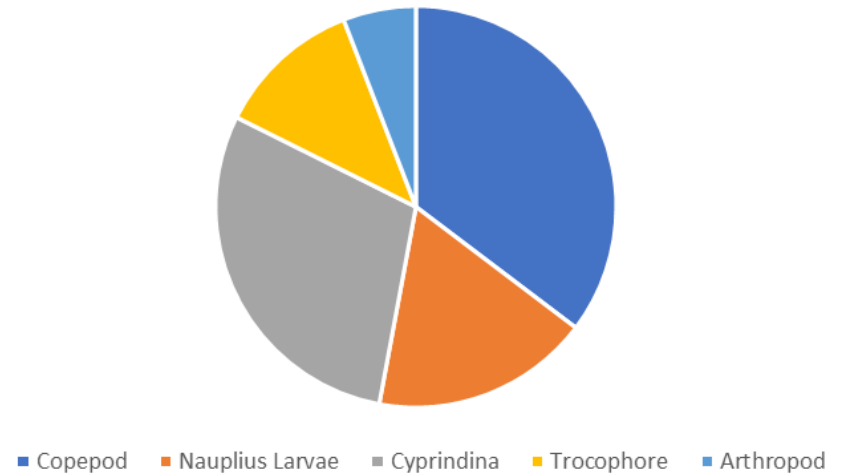
Plankton Speciation
