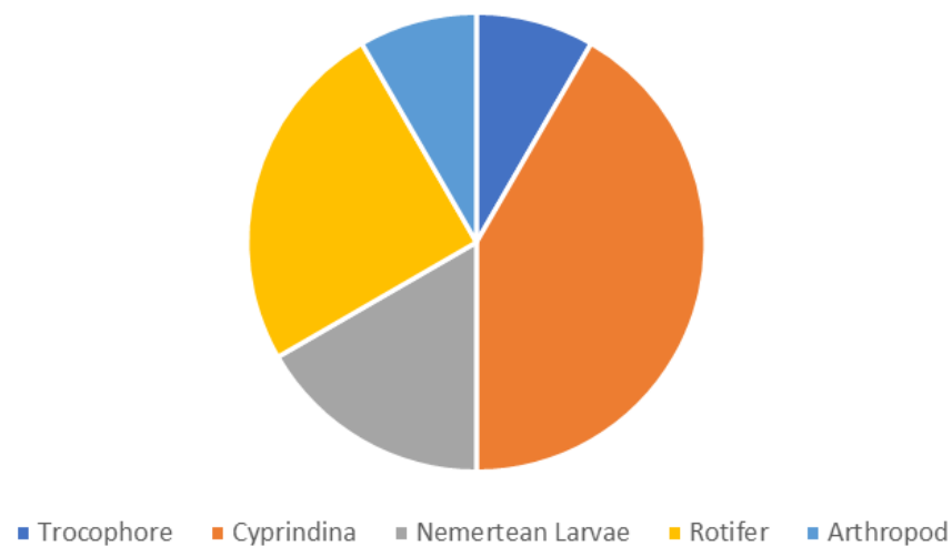
Plankton Speciation
