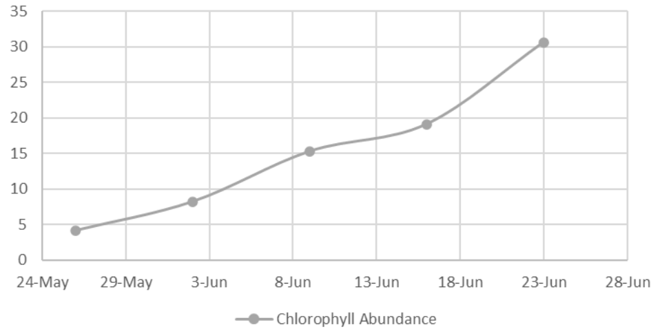
Chlorophyll Abundance
