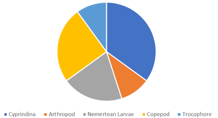
Plankton Speciation
