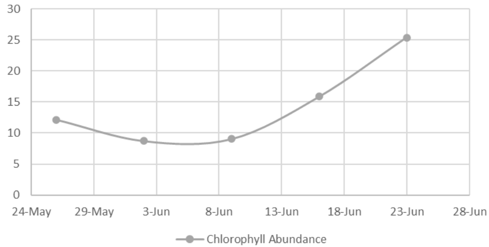
Chlorophyll Abundance
