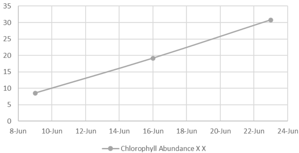
Chlorophyll Abundance
