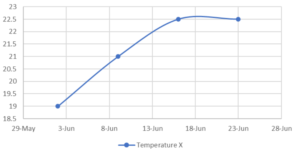
Temperature
