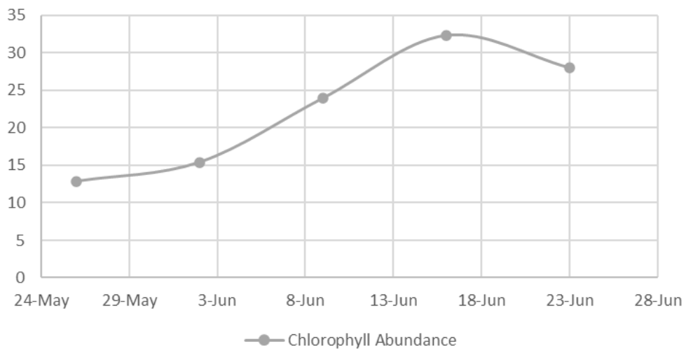
Chlorophyll Abundance
