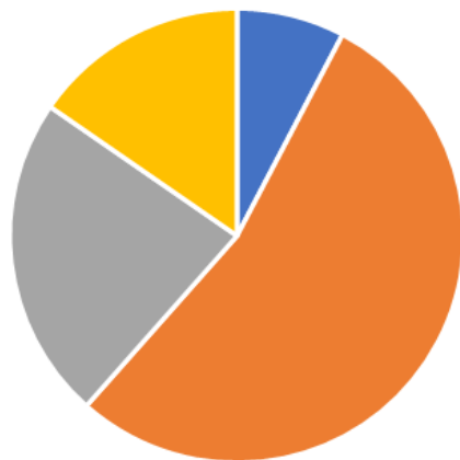
Plankton Speciation
