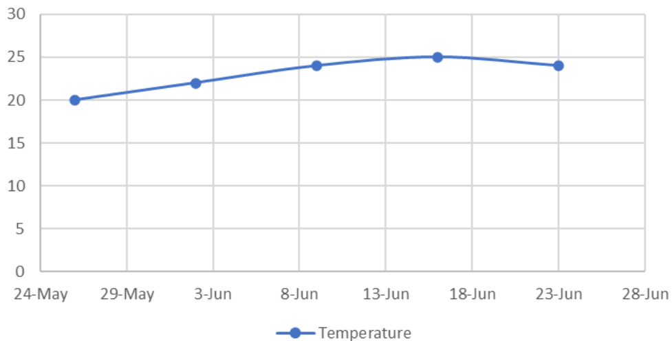
Temperature
