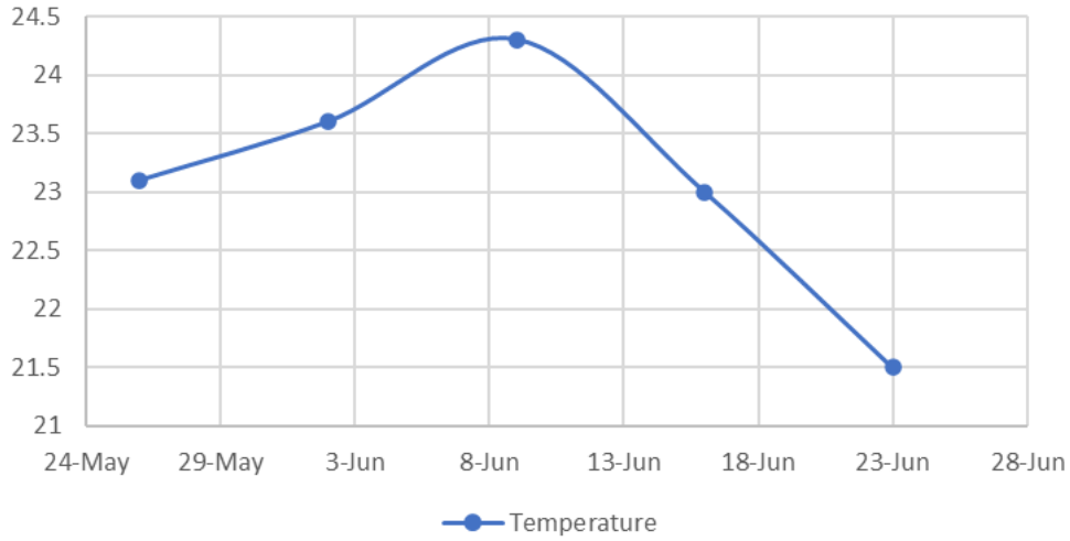
Temperature
