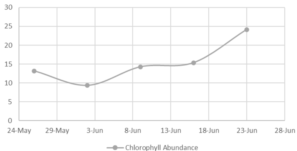
Chlorophyll Abundance
