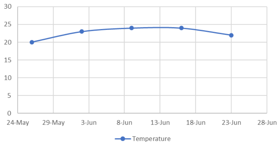
Temperature
