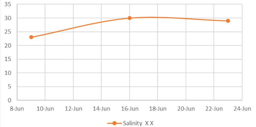
Salinity
