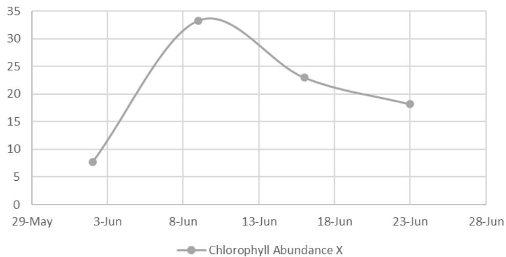
Chlorophyll Abundance
