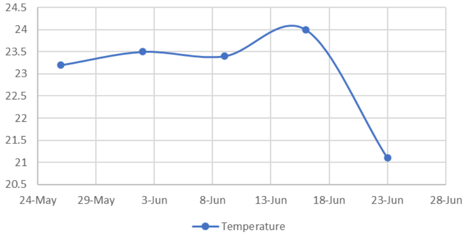
Temperature
