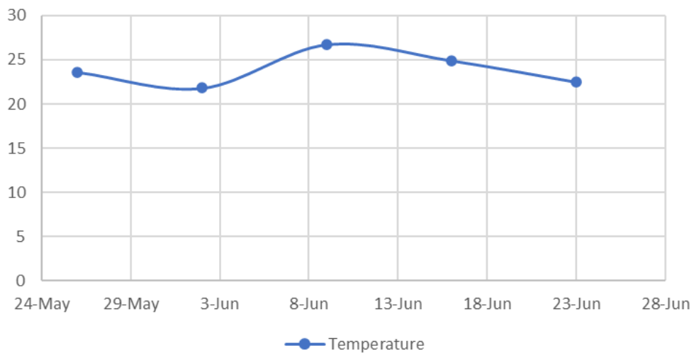
Temperature
