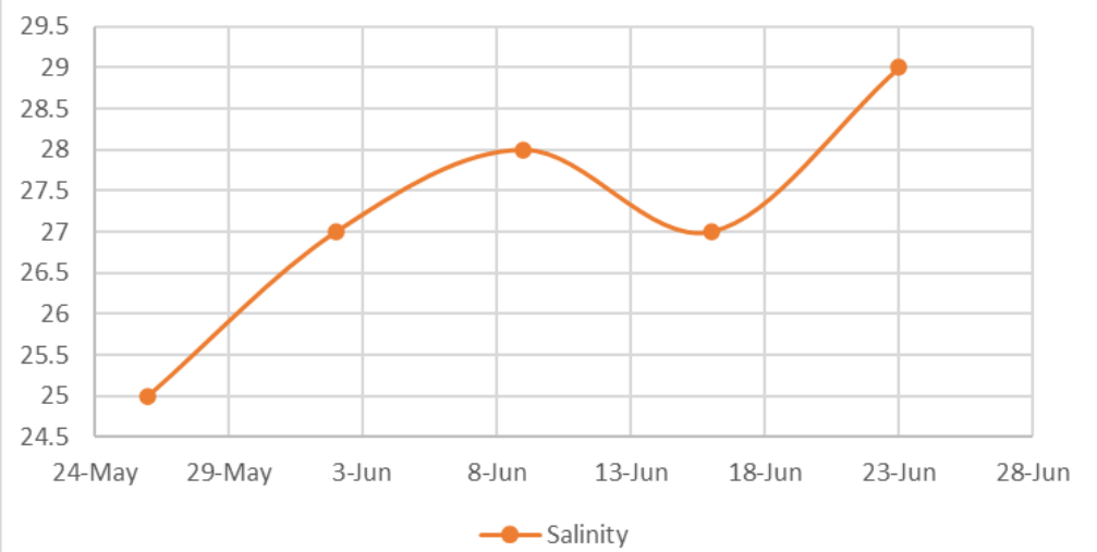
Salinity
