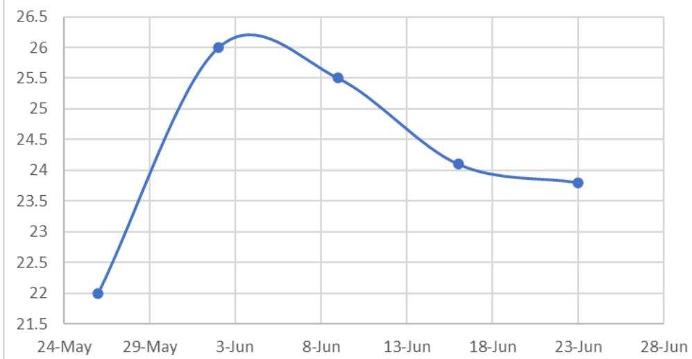
Temperature
