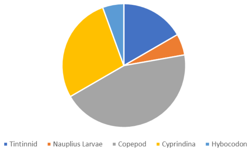
Plankton Speciation
