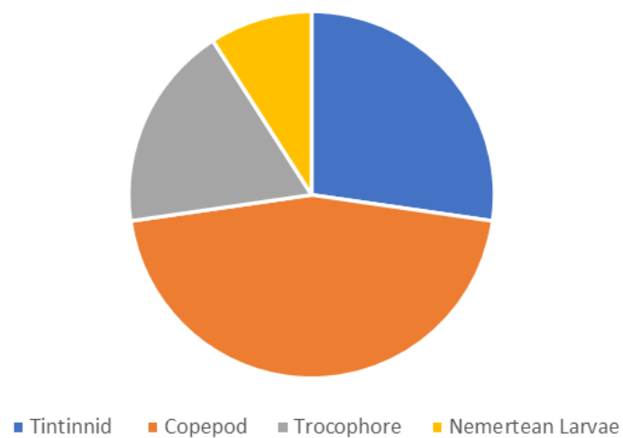
Plankton Speciation
