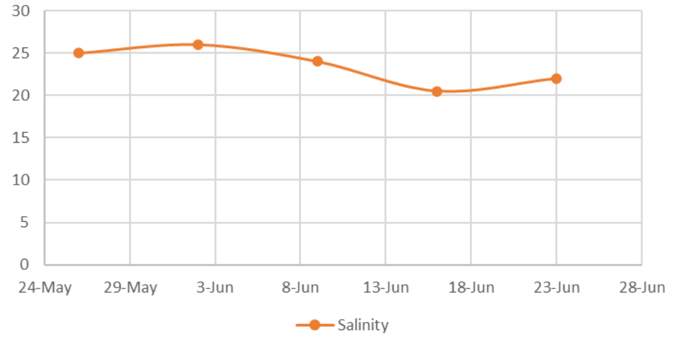
Salinity
