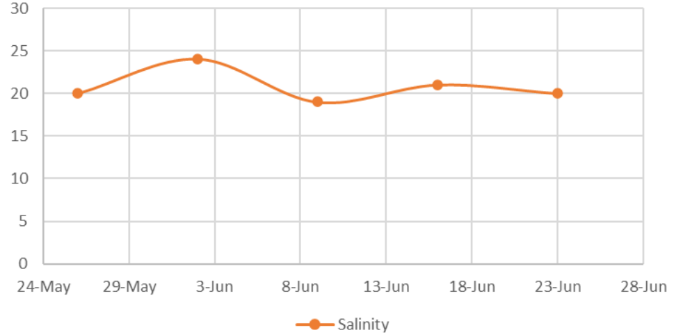
Salinity
