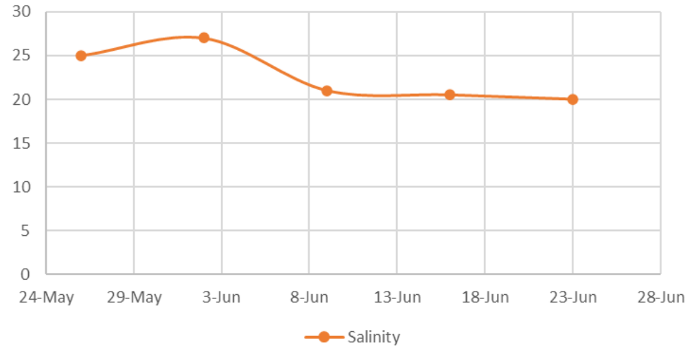
Salinity
