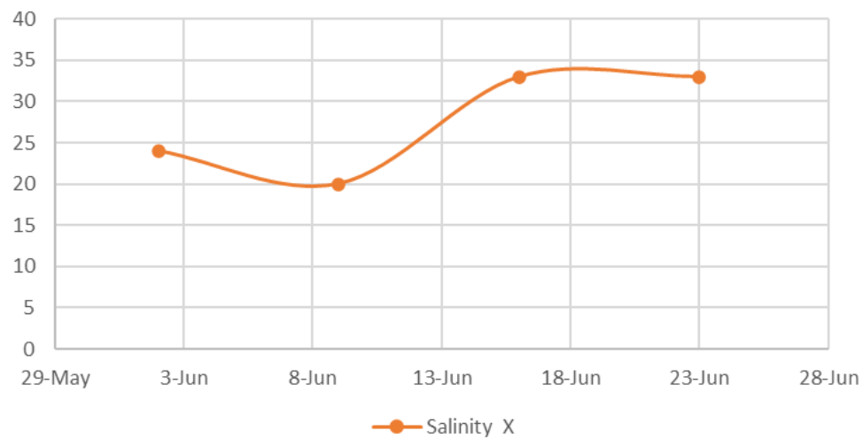
Salinity
