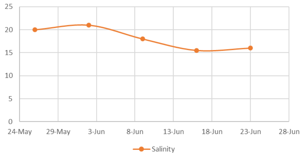
Salinity
