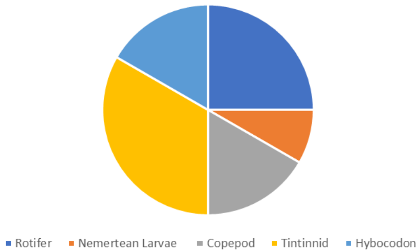
Plankton Speciation
