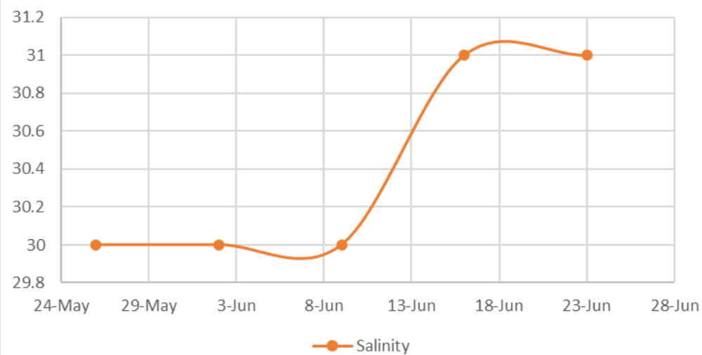
Salinity
